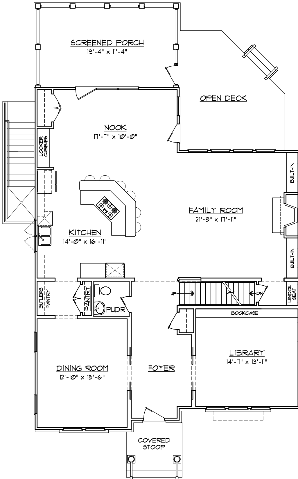
FIRST FLOOR PLAN for LOT "4" LIVE OAK DRIVE
